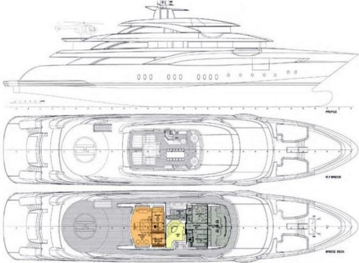
72 GOLD - BRIDGE DECK ACCOMODATION, FLY BRIDGE & PROFILE - SCALE 1:200
